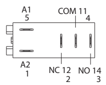
Cat. No. 700-HK36_ (SPDT)
