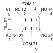
Cat. No. 700-HK32_ (DPDT)
